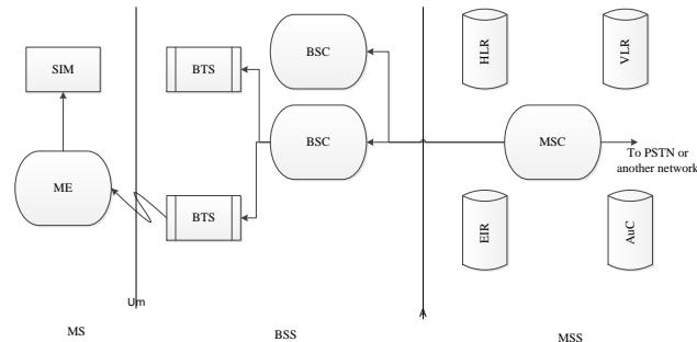
Figure 1. GSM Network Architecture
