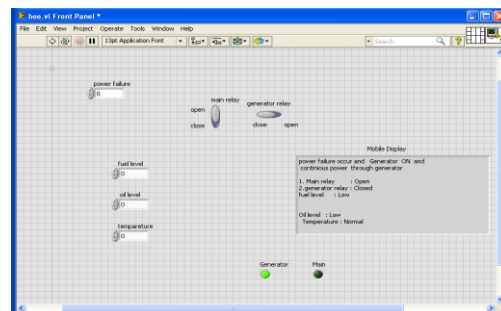
Figure 5. Continous Power through Generator Status
