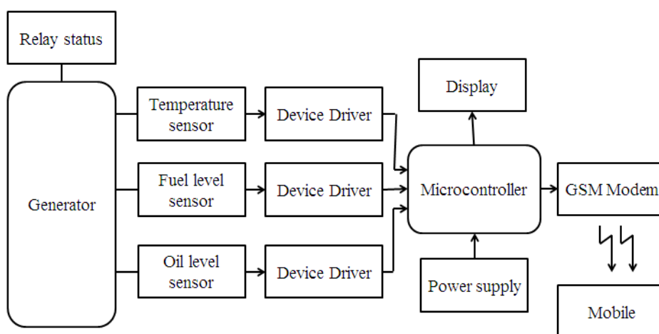
Figure 2. Block Diagram of Proposed System
