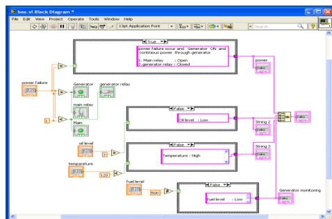
Figure 4. Block Diagram of Simulation Model
