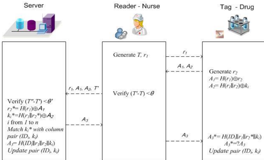
Figure 2. Authentication Phase of New Proposed Protocol
