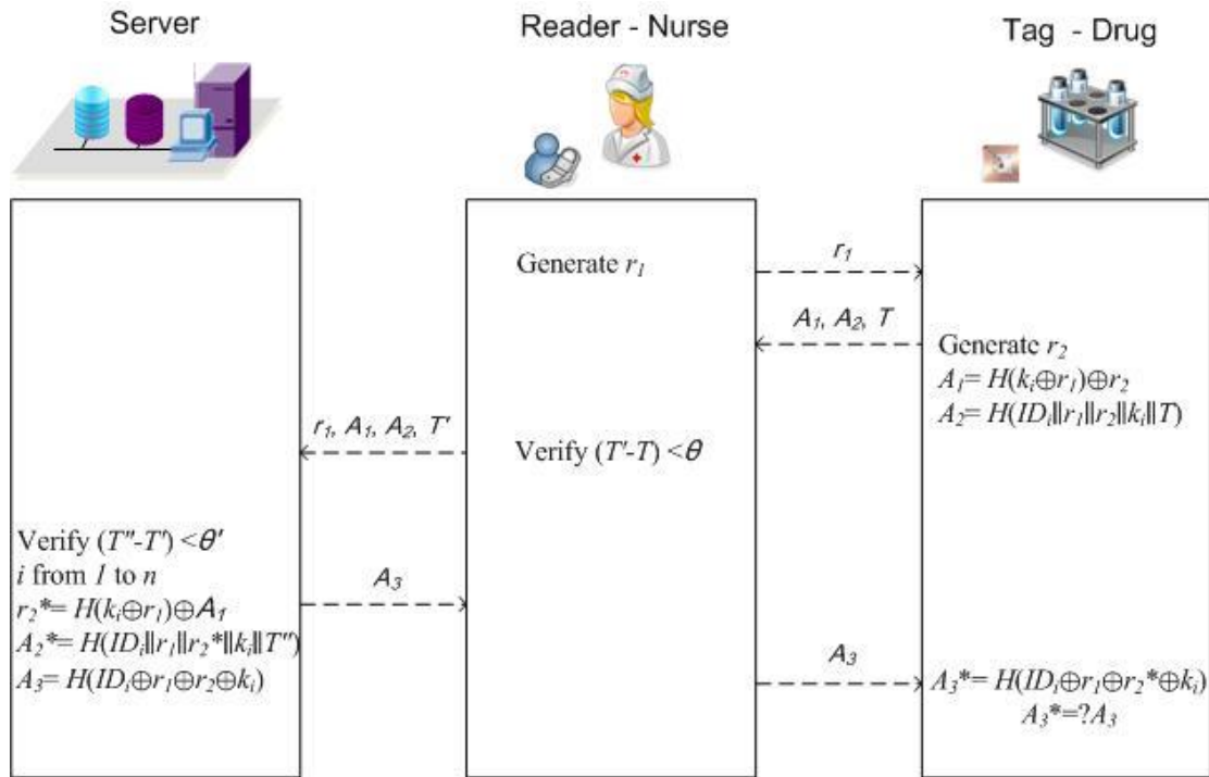
Figure 1. Authentication Phase of This Protocol
