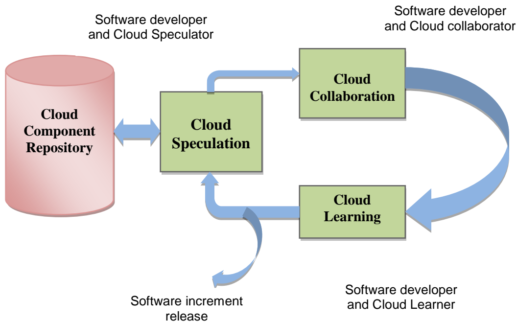
Figure 7. Adaptive Cloud Development (ACD) Model
