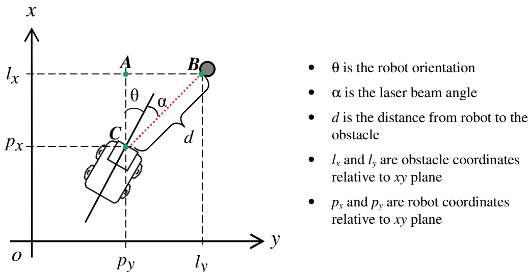
Figure 3. Laser beam decomposition in xy surface
