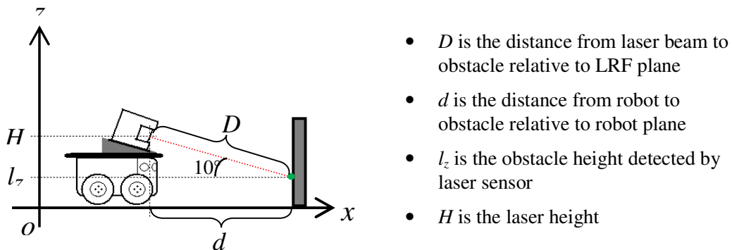
Figure 2. Laser beam decomposition in zx surface.
