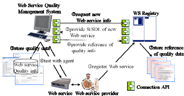
Figure 4. Scenario 1: Quality Data Registration
