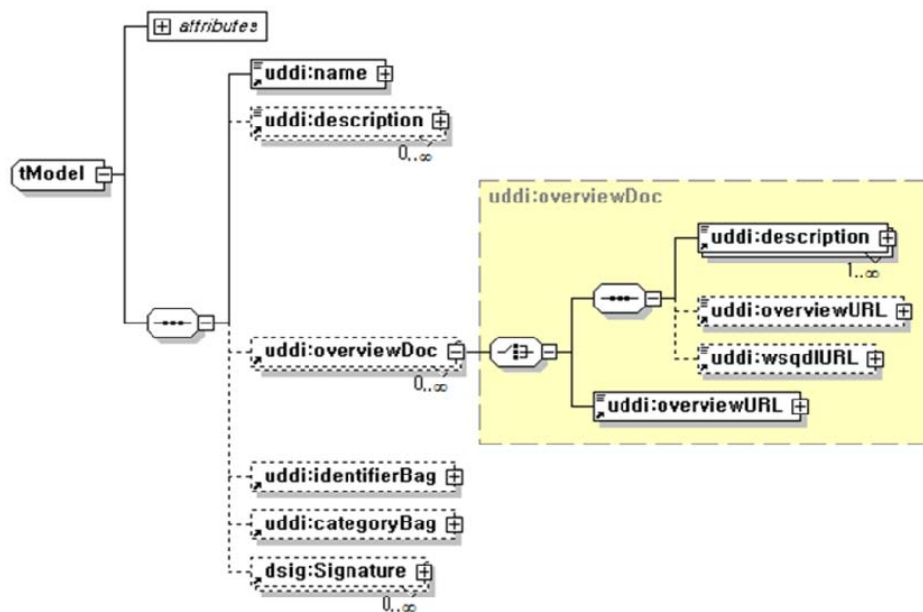
Figure 5. tModel and its Schema including <wsqdlURL> component
