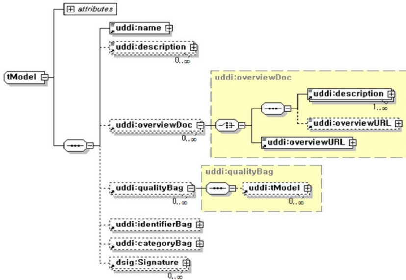
Figure 6. tModel Component and Schema including qualityBag
