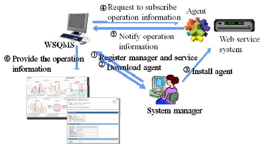
Figure 1. Web Service Monitoring Process
