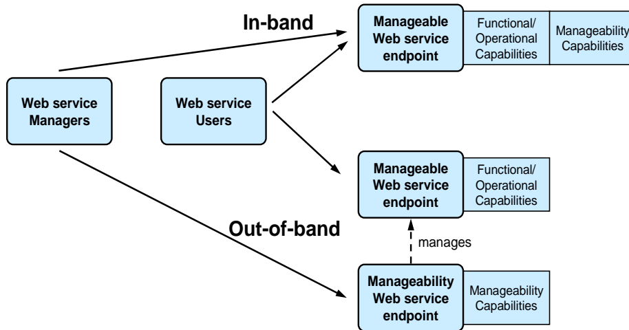
Figure 2. WSQMS Agent Type
