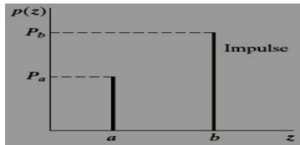
Figure 5. PDF Plot of Salt and Pepper Noise
