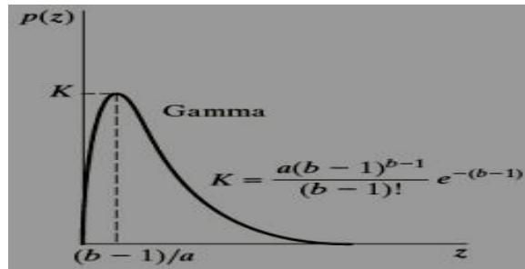
Figure 2. PDF Plot of Gamma Noise
