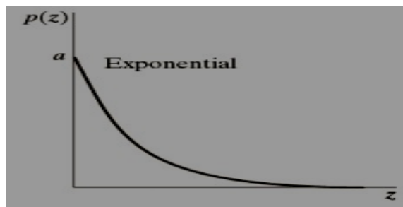
Figure 3. PDF Plot of Exponential Noise
