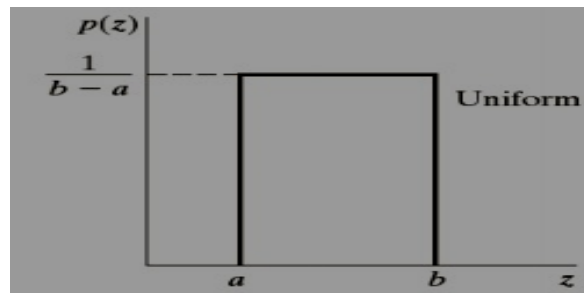
Figure 4. PDF Plot of Uniform Noise
