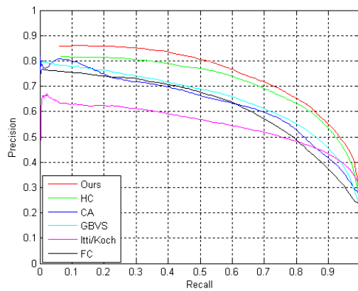
Figure 6. Comparison of Precision-recall Curves of Saliency Maps
