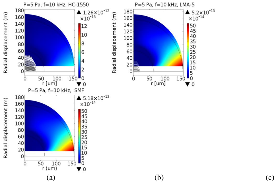
Figure 2. Radial Displacement Profile for (a) HC-1550, (b) LMA-5, and (c) SMF, for p = 5 Pa, f = 10 kHz.
