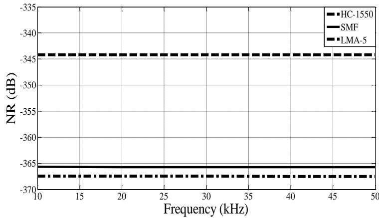
Figure 5. Average NR as a Function of Acoustic Frequency for the HC-1550, LMA-5, and SMF for Acoustic Pressure of 1 Pa
