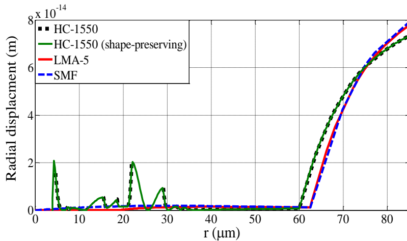
Figure 3. Radial Displacement as a Function of Fiber Radius for (a) HC-1550, (b) LMA-5, and (c) SMF, for p = 5 Pa, f = 10 kHz
