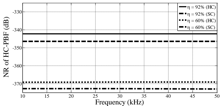
Figure 6. NR of HC-PBF as a Function of the Acoustic Frequency for Different Air-Filling Ratios (HC) Indicates using the Same Structure with Hollow-core, while (SC) Indicates using the Same Structure with Solid-Core
