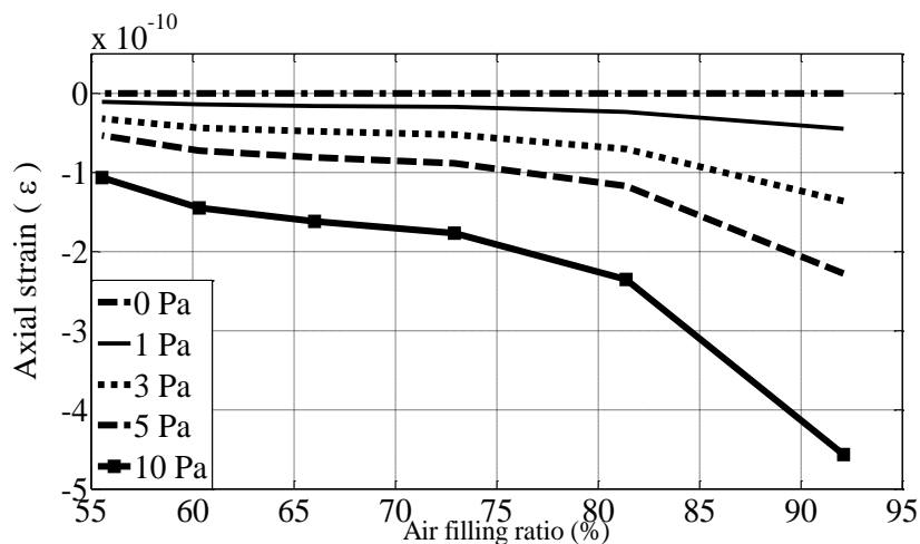
Figure 4. Axial Strain of the Microstructured Region of HC-1550 as a Function of \eta for Different Acoustic Pressures
