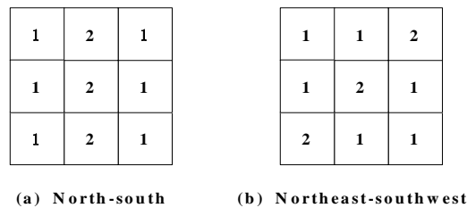
Figure 1. The Weights Strategy of the Adjacent Pixels of Spatial Filtering
