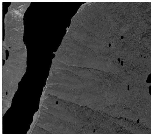
Figure 5. The Potential Landslide Region Extracted with Thresholding
