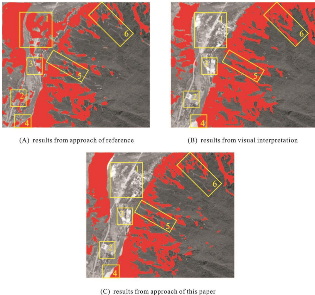
Figure 7. Landslide Region Extracted from this Three Approaches
