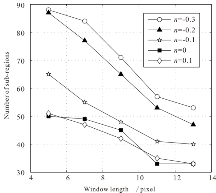
Figure 6. The Relationship between the Filtering Window Length and Number of Landslide Sub-regions
