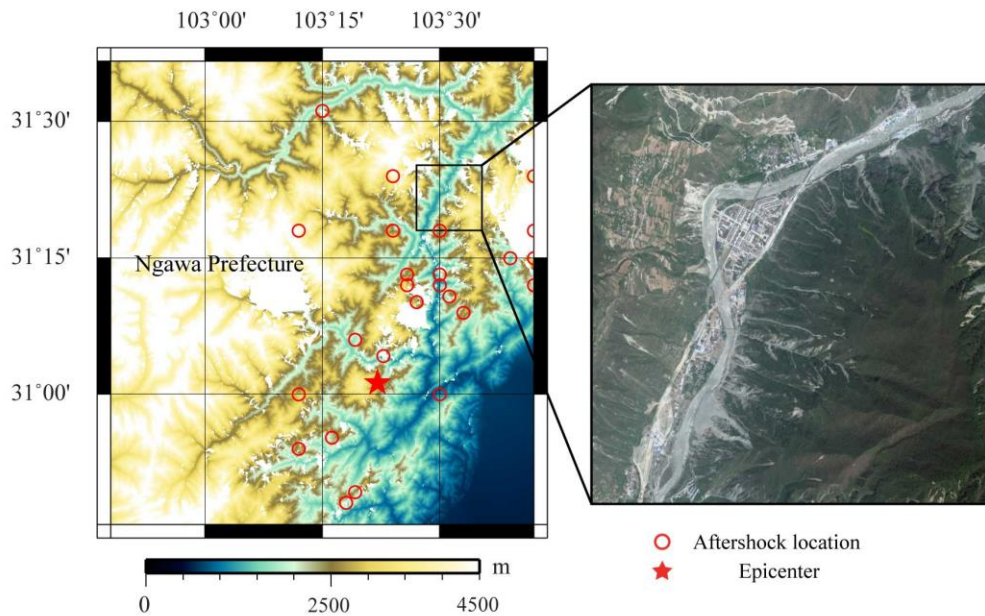
Figure 2. Basic statues of Wenchuan County and AOI
