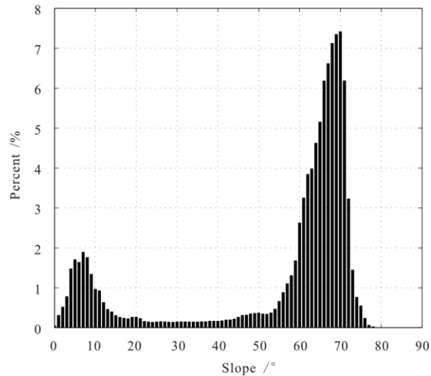
Figure 4. Statistics of the Slope Distribution
