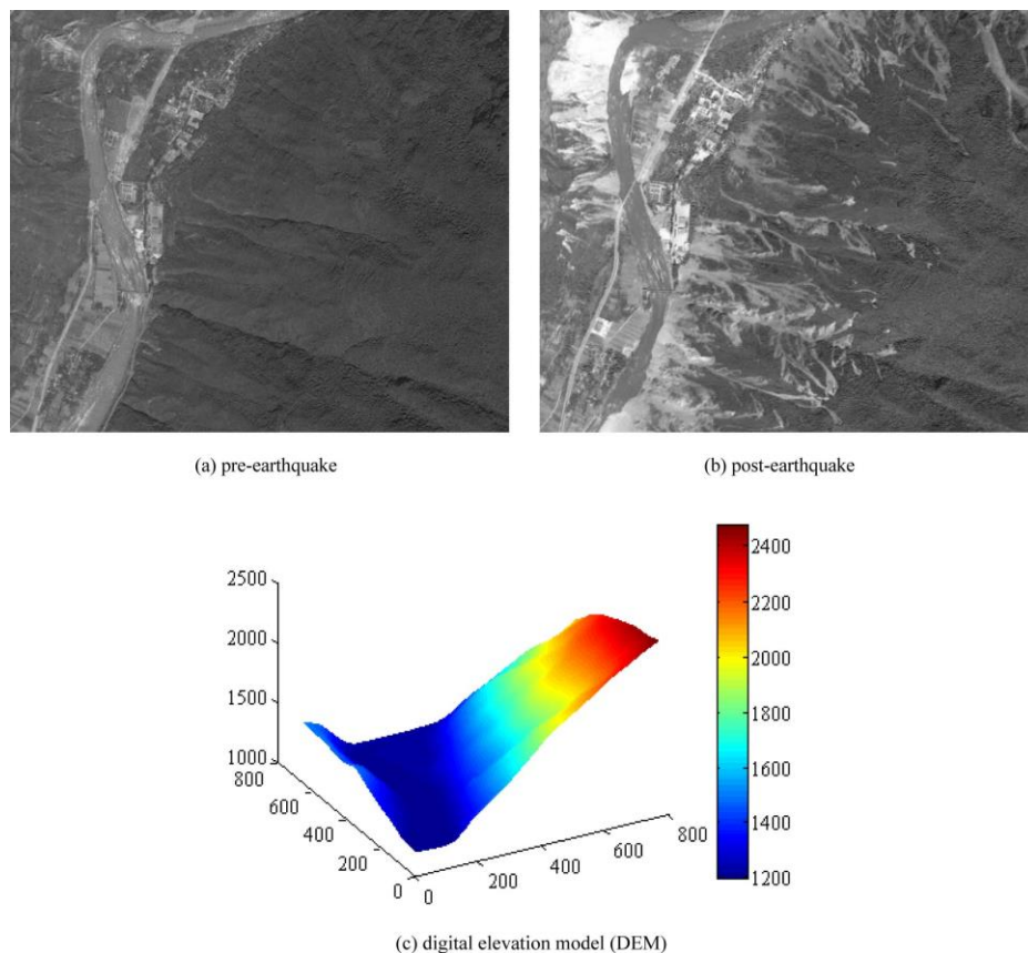
Figure 3. The Preprocessed Satellite Images and DEM
