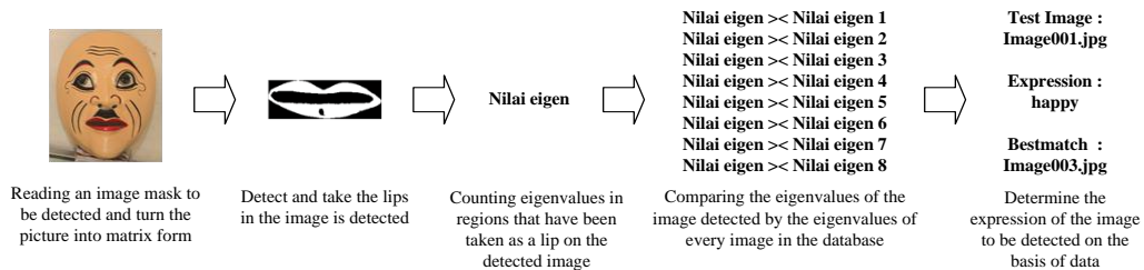
Figure 4. Expression Detection Process
