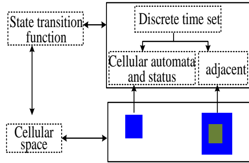
Figure 3. Agent Structure
