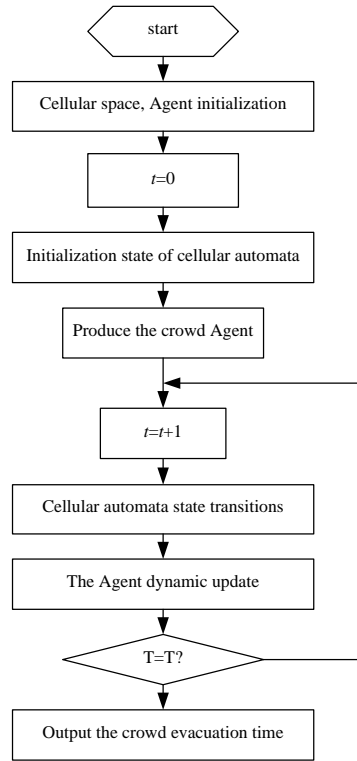
Figure 5. Flow Chart of Agent-CA Algorithm
