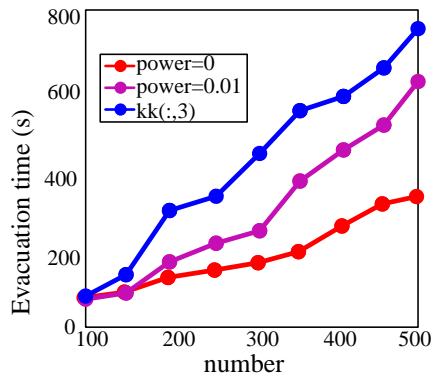
Figure 7. Impact of the Physical Value on Evacuation Behavior
