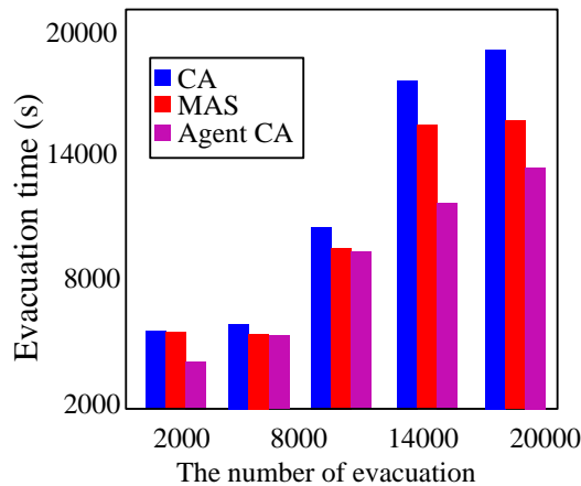
Figure 9. Performance Comparisons of Different Stadium Crowd Evacuation Models
