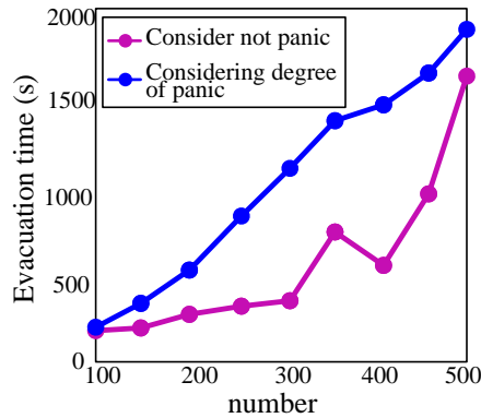
Figure 8. Impact of the Level of Panic on Evacuation Behavior
