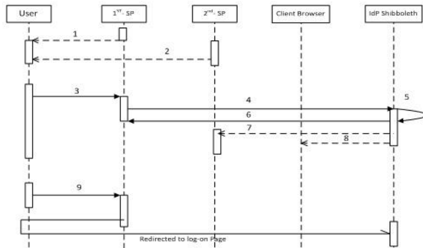
Figure 8. Proposed Logout Sequence Diagram
