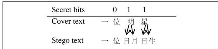
Figure 2. An Example of Wang’s Text Hiding Scheme
