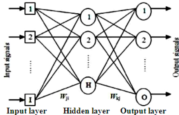
Figure 2. Three Layer ANN Architecture
