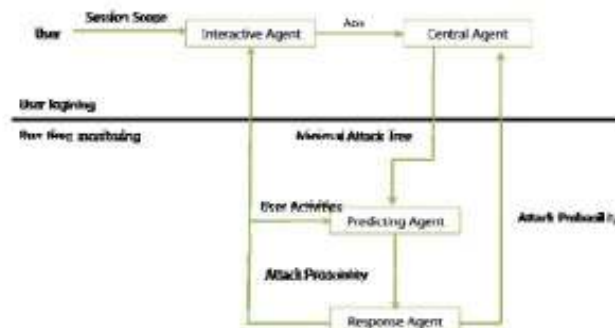
Figure 4. Flow diagram for insider threat model
