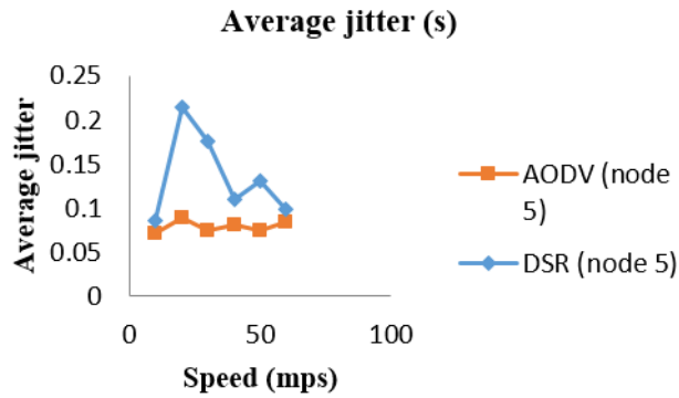
Figure 4. Average Jitter for AODV and DSR (Node 5)
