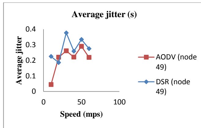
Figure 5. Average Jitter for AODV and DSR (Node 49)
