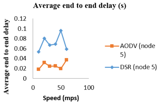
Figure 3. Average End to End Delay for AODV And DSR(Node 5 )
