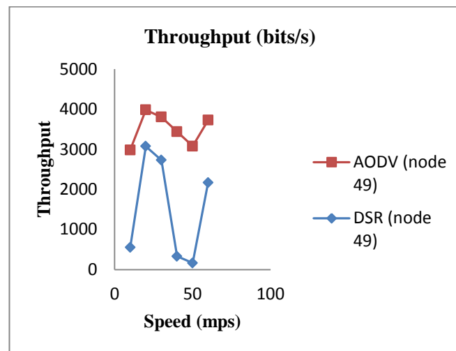
Figure 7. Throughput for AODV and DSR (Node 49)
