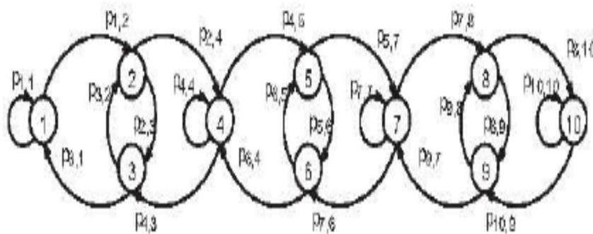
Figure 8. Discrete Markov Model for the Handover Succession without Hysteresis
