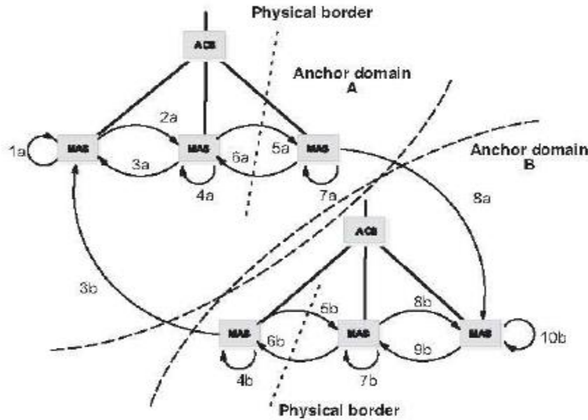
Figure 9. Handover between Neighboring Domains with Hysteresis
