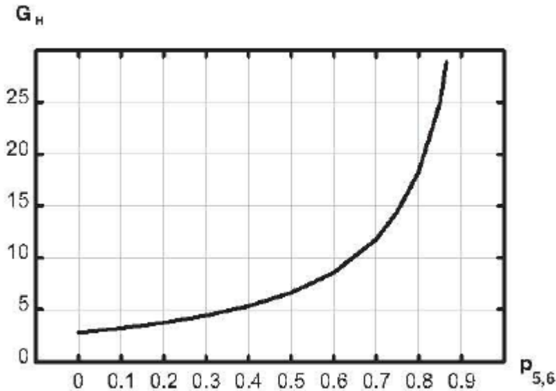
Figure 11. Hysteresis Gain
