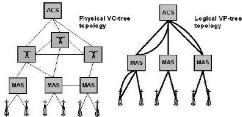
Figure 4. MN-A VP Topology
