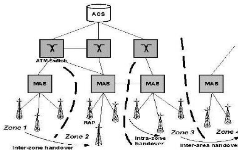
Figure 1. Architecture of the Wireless ATM Network
