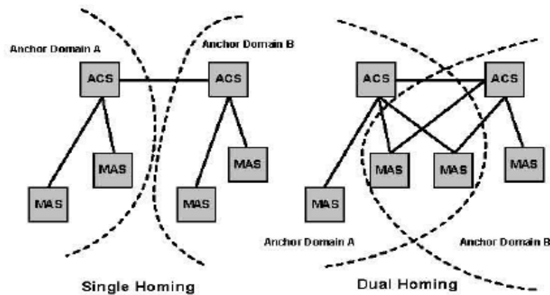
Figure 6. VP based Dual Homing
