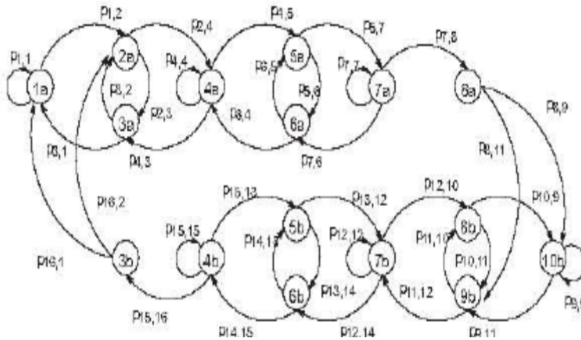
Figure 10. Discrete Markov Model for the Handover Succession with Hysteresis
