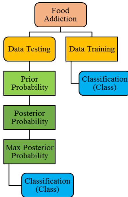
Figure 3. Naïve Bayes Model
