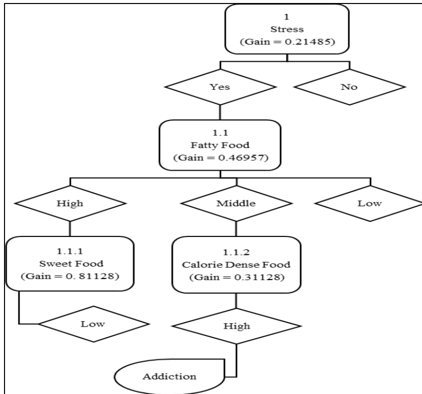
Figure 6. Decision Tree Classification
