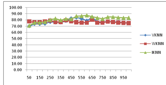
Figure 5. Micro-averaged F1 Measure on WebKB dataset
