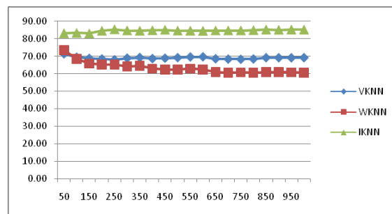
Figure 4. Micro-averaged F1 Measure on Reuters dataset
