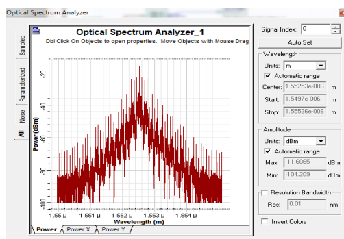
Figure 8: Response Of DPSK Transmitter Before Including Amplitude Noise And Phase Noise
