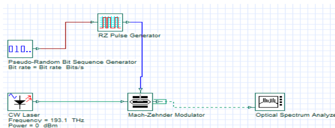
Figure 2: PSK Optical Transmitter in Optisystem
