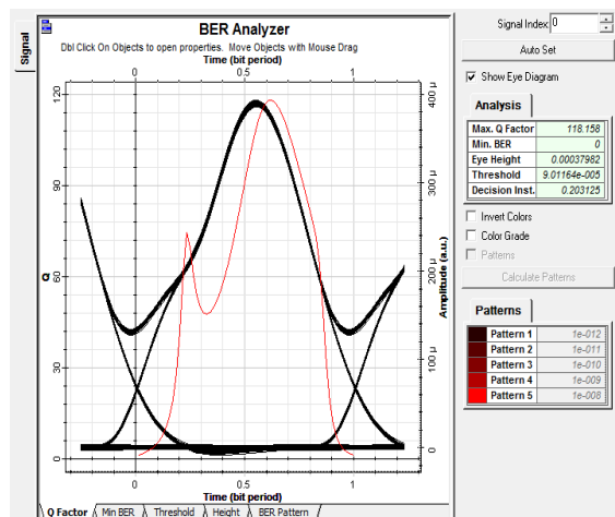
Figure 11: BER After Applying All Optical Regeneration Using 3R And PSA
