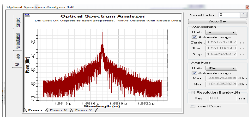
Figure 7: Response of DPSK Transmitter
