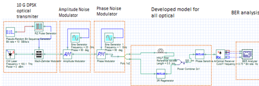
Figure 6: Developed Model For All Optical Regeneration Using 3R And PSA
