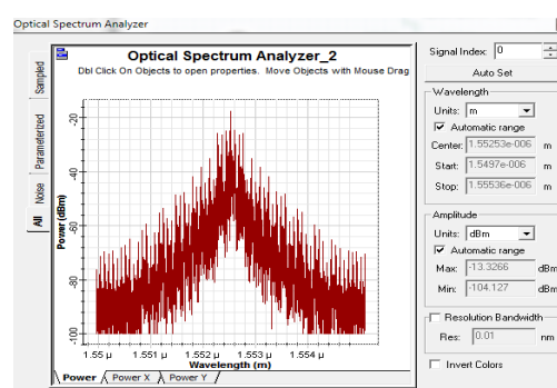
Figure 9: Response Of DPSK Transmitter After Including Amplitude Noise And Phase Noise
