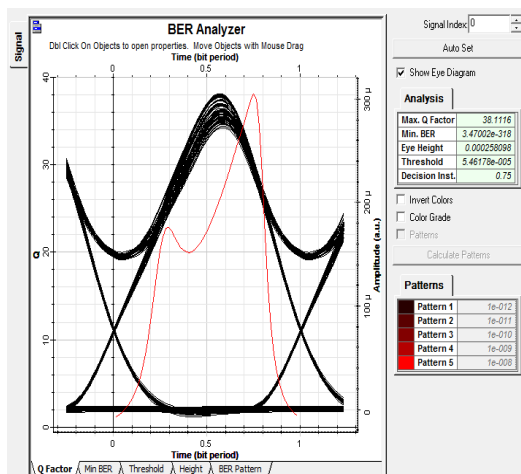
Figure 10: BER Before Applying All Optical Regeneration Using 3R And PSA
