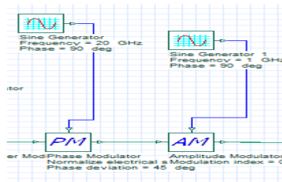
Figure 4: Noise Emulator In Optisystem
