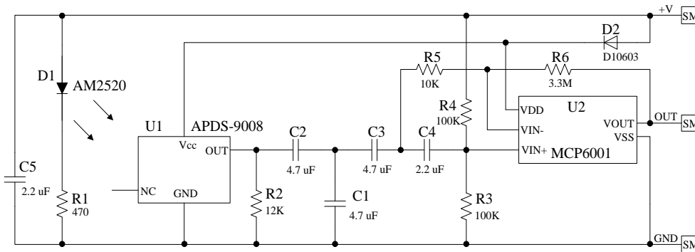
Figure 4. Pulse Sensor Circuit Diagram
