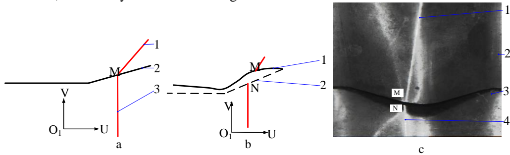
Figure 2. The Laser Projection Line: (a) AG-W without Gap: 1. The Laser Line Projected on the Corrugated Sheet, 2. The Edge of the Corrugated Sheet, 3. The Laser Line Projected on the Base Plate, (b) The Existing Gap in AG-W: 1. The Actual Edge of the Corrugated Sheet, 2. The Theoretical Edge of the Corrugated Sheet, (c) The Laser Projection Line with Gap: 1. The Laser Line Projected on the Corrugated Sheet, 2. The Corrugated Sheet, 3. The Base Plate, 4. The Laser Line Projected on the Base Plate
