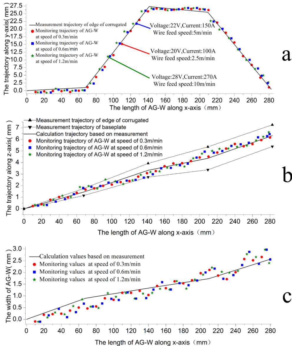
Figure 8. The Gap Width of AG-W and Trajectory of the AG-W: (a) The Trajectory of AG-W along the y-axis, (b) The Trajectory of AG-W along the z-axis, (c) The Gap Width of AG-W
