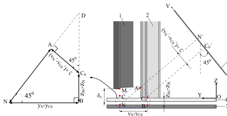
Figure 5. The Principle of Acquiring the Actual Trajectory of Centerline of AG-W along y -axis: 1. The Actual Position of the Corrugated Sheet, 2. The Theoretical Position of the Corrugated Sheet, 3. The UV Imaging Plane, 4. The Theoretical Position of the Base Plate, 5. The Actual Position of the Base Plate
