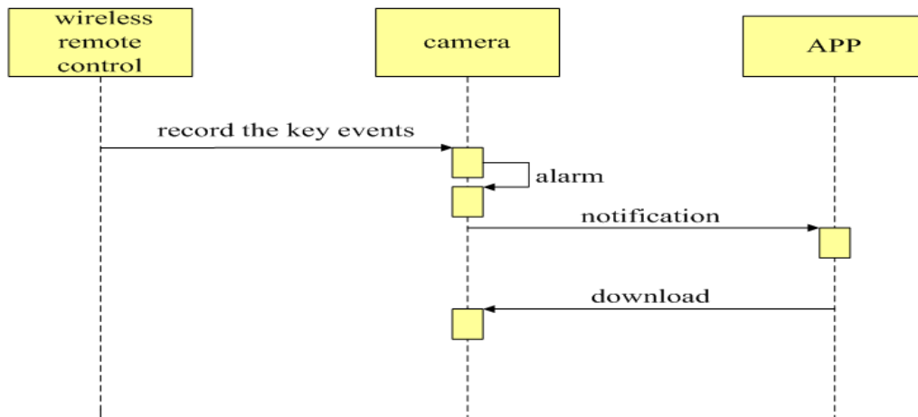
Figure 9. Key Event Log Process
