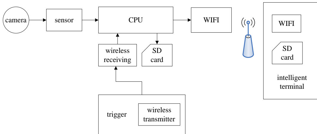
Figure 1. Overall Structure
