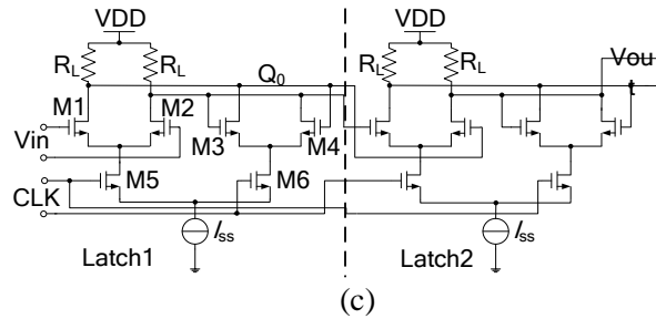
Figure 2. The CML-based Circuit. (a) Summer; (b) MUX; (c) MSDFF
