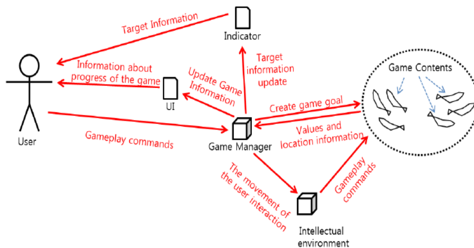
Figure 3. Immersive Virtual Reality Game Play Flow Chart
