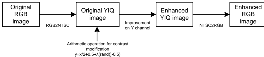
Figure 1. Proposed contrast intensification pipeline
