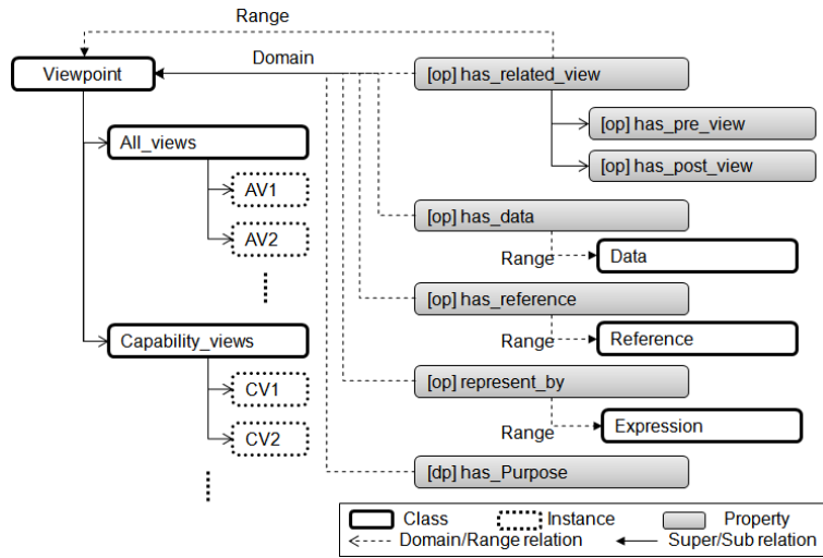
Figure 3. Overall Relationships among ‘Viewpoint,’ ‘View,’ their Properties, and Instances
