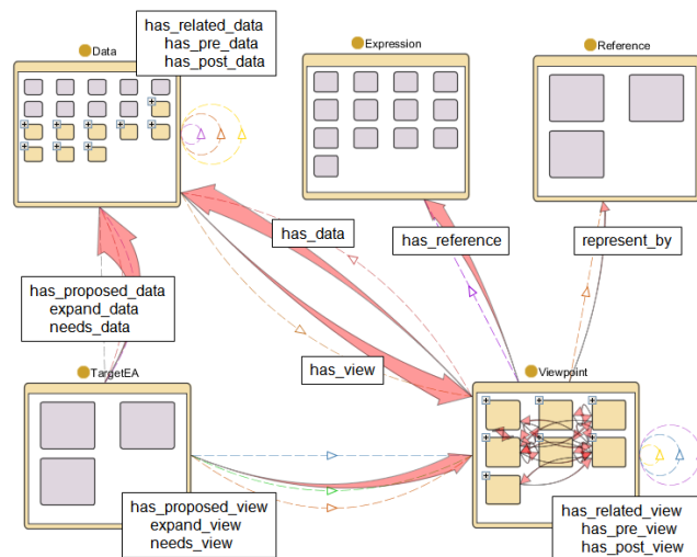
Figure 2. Overall Structure of ONT-DAF
