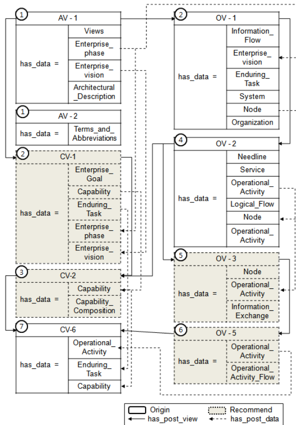
Figure 4. Inference Result of ONT-DAF
