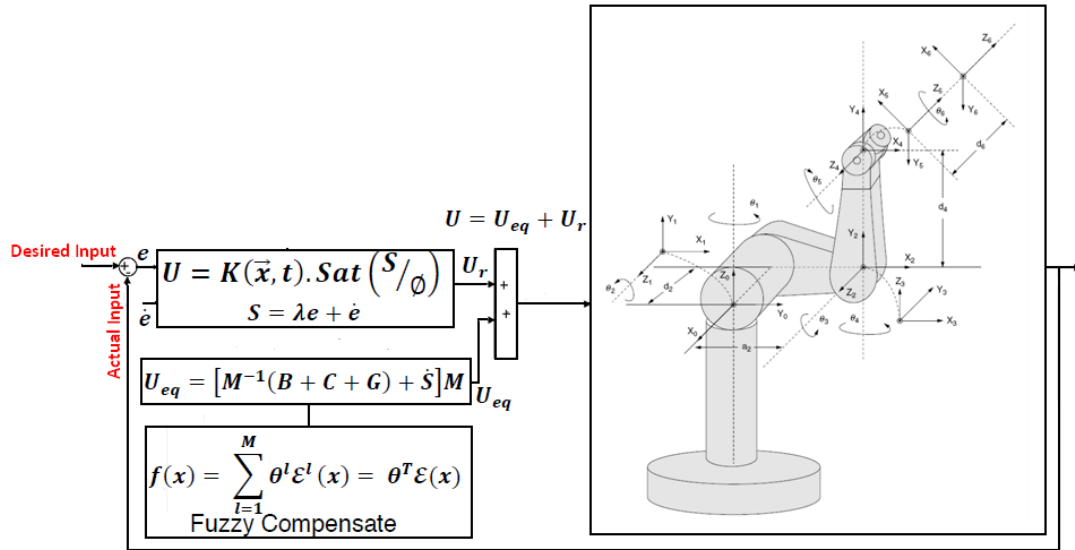
Figure 3: Chattering free Block diagram of a fuzzy estimator variable structure controller
