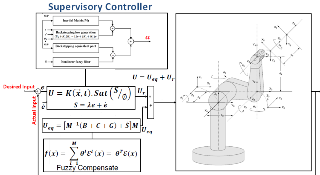
Figure 4: Chattering free Block diagram of a SISO fuzzy backstepping adaptive fuzzy estimator variable structure controller
