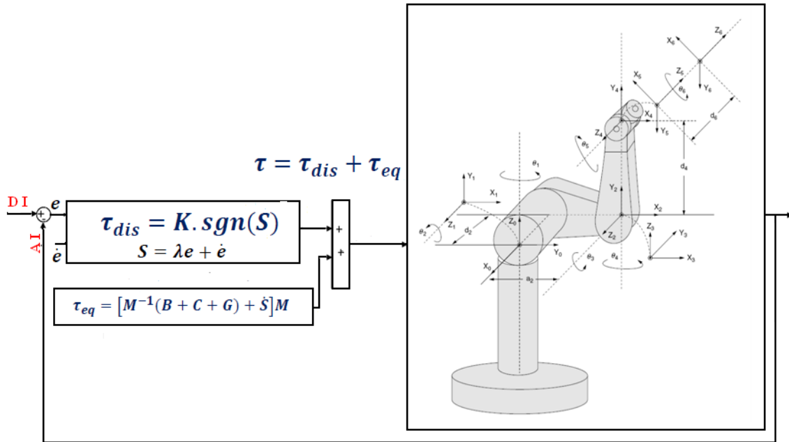
Figure 1: Block Diagram of a Variable Structure Controller: Applied to Robot Arm
