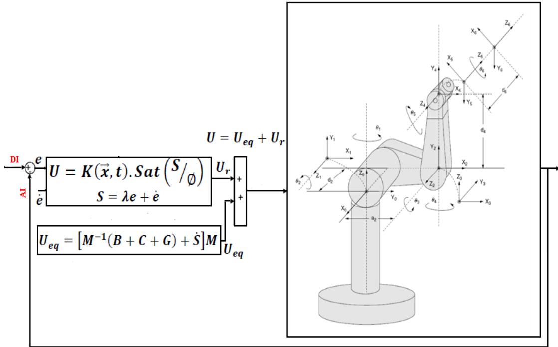
Figure 2: Chattering Free Block Diagram of a Variable Structure Controller: Applied to Robot Arm
