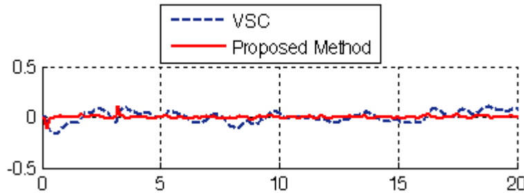
Figure 7: VSC Vs. SISO fuzzy backstepping adaptive fuzzy estimator variable structure controller: Robot arm steady state error in presence of external disturbance
