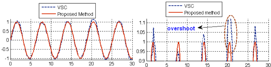
Figure 6: VSC Vs. SISO fuzzy backstepping adaptive fuzzy estimator variable structure controller: Robot arm with external disturbance
