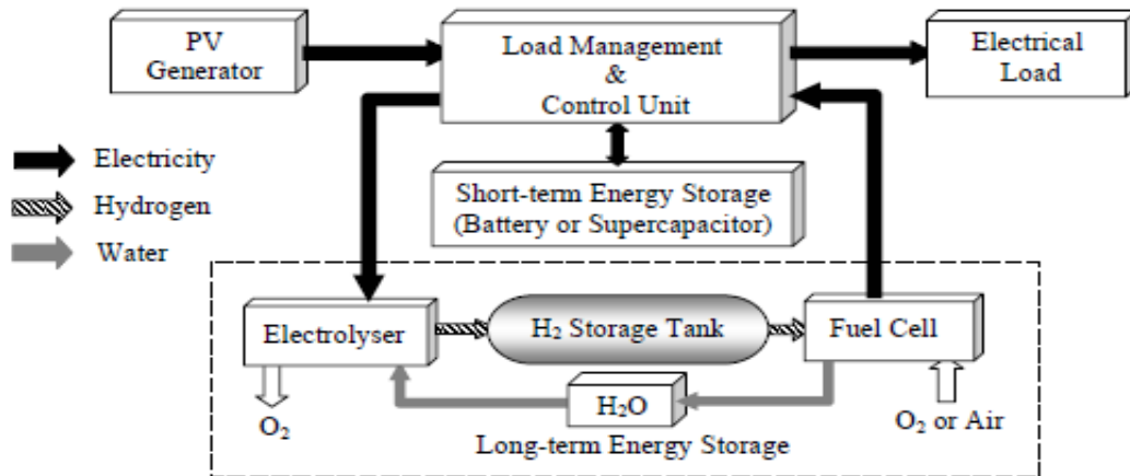
Figure 3. Block Diagram of Fuel Cell and Renewable Hydrogen Energy System
