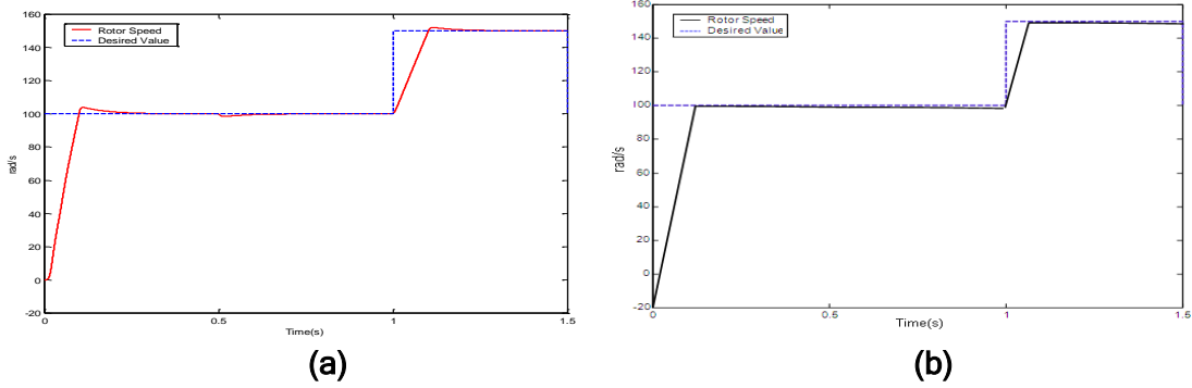
Figure 12. Regulated Speed: PFLC (a) vs [2] (b)
