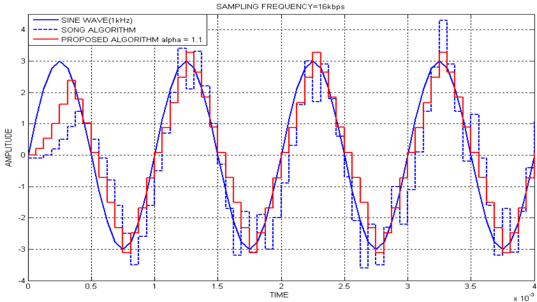
Figure 5. Performance comparison of SONG algorithm with Proposed Algorithm.
