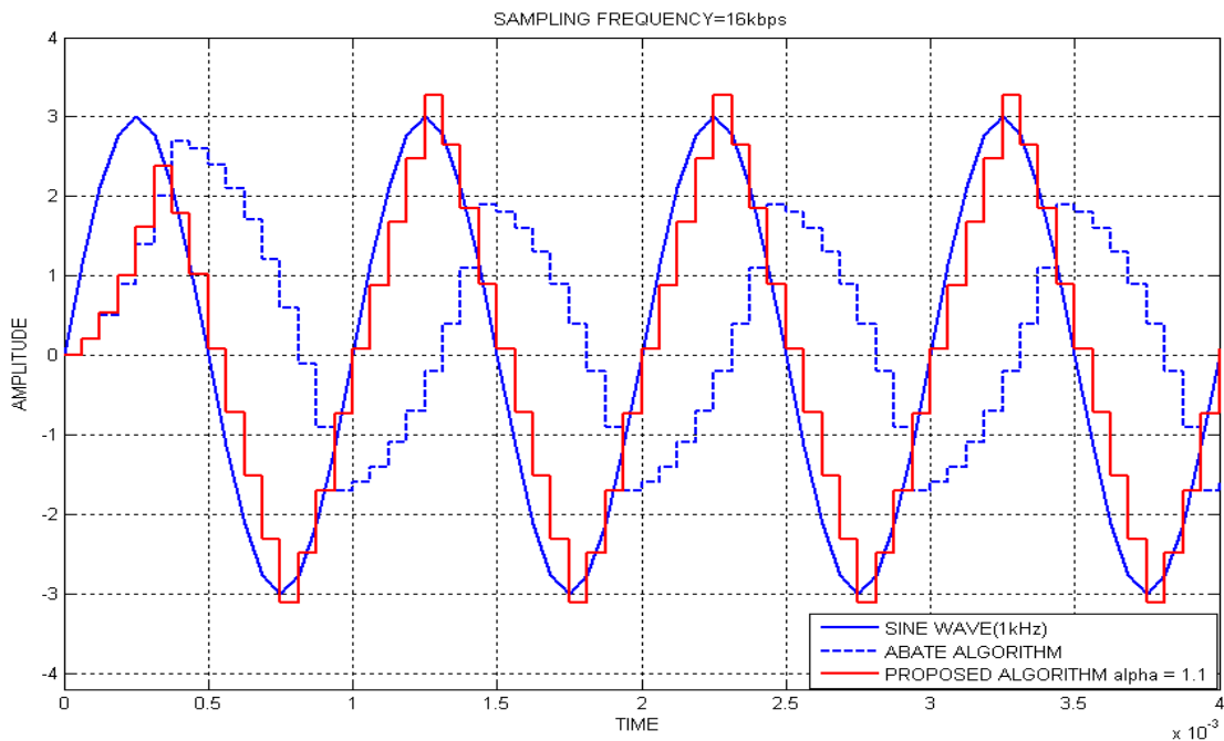
Figure 6. Performance comparison of ABATE algorithm with Proposed Algorithm.
