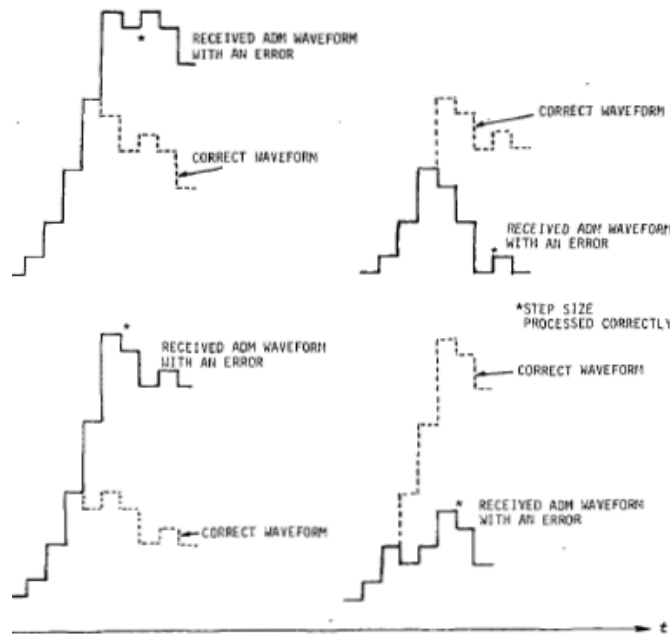
Figure 4. Modified-ABATE waveforms with channel errors showing step size recovery
