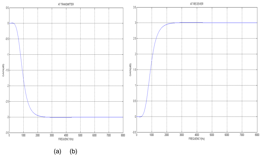
Figure 10. (a). Frequency response of Pre-Processor (Integrator) at the transmitter (b). Frequency response of the Differentiator at the receiver.
