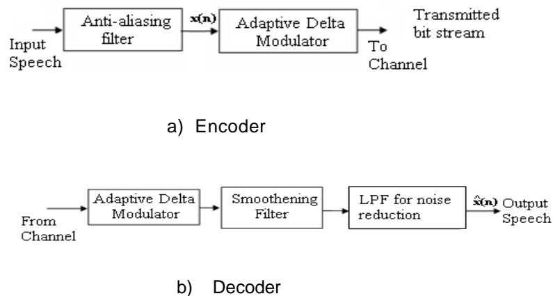
Figure 8. The block diagram of Conventional ADM
