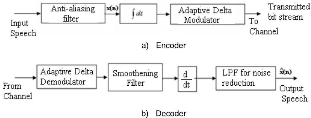
Figure 9. The block diagram of proposed ADM
