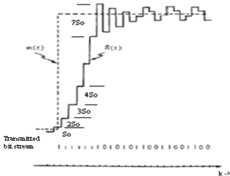
Figure 3. Adaptive delta modulation showing the changing step size and bit pattern produced using SONG algorithm.
