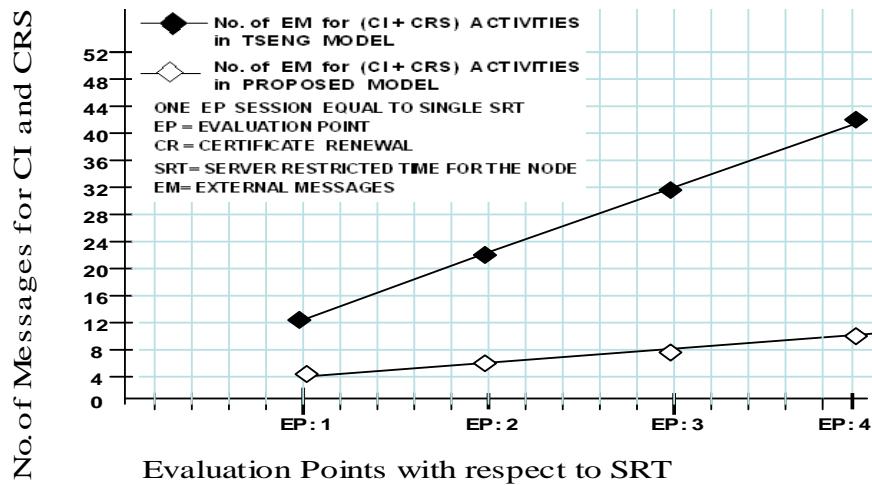
Fig. 12. Number of External Messages for CI and CRS at EPs
