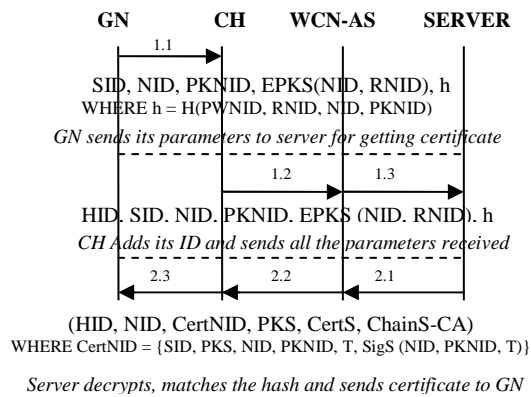
Fig. 11. Exchange of Messages in Tseng Model
