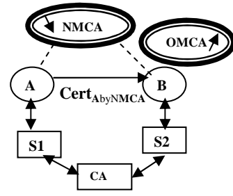
Fig. 8. NMCA replaces OMCA in NSDS
