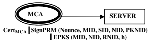
Fig. 2. Verification from Server
